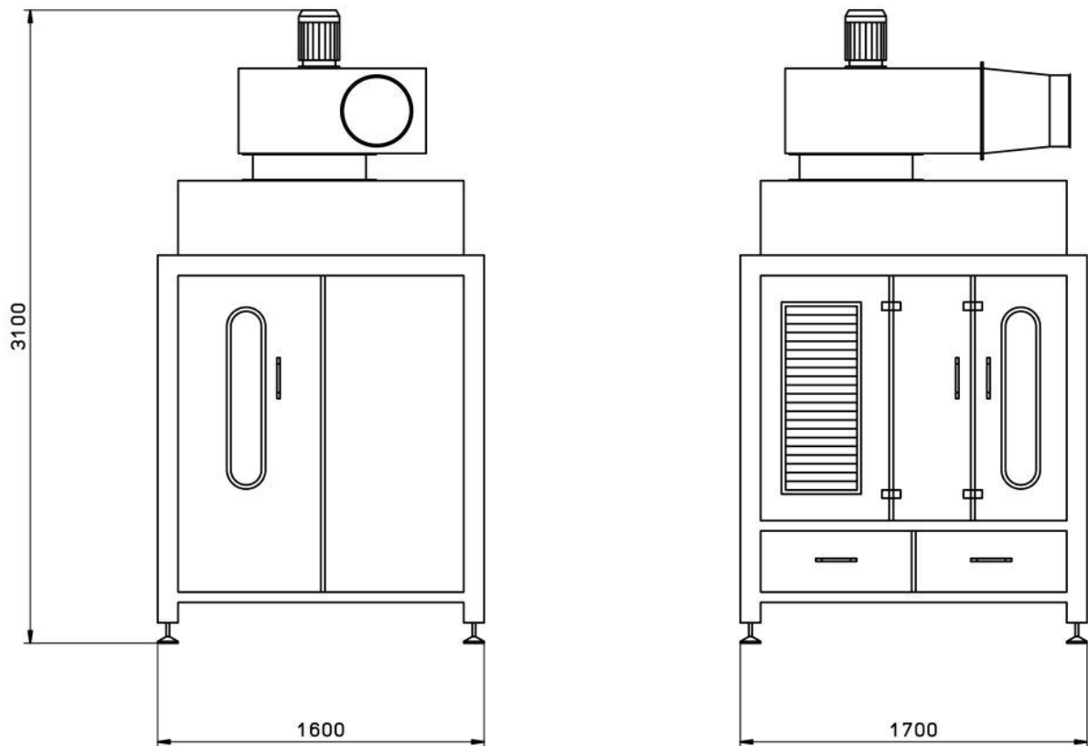
Dimensions of the machine in service Net weight: 780 kgs
